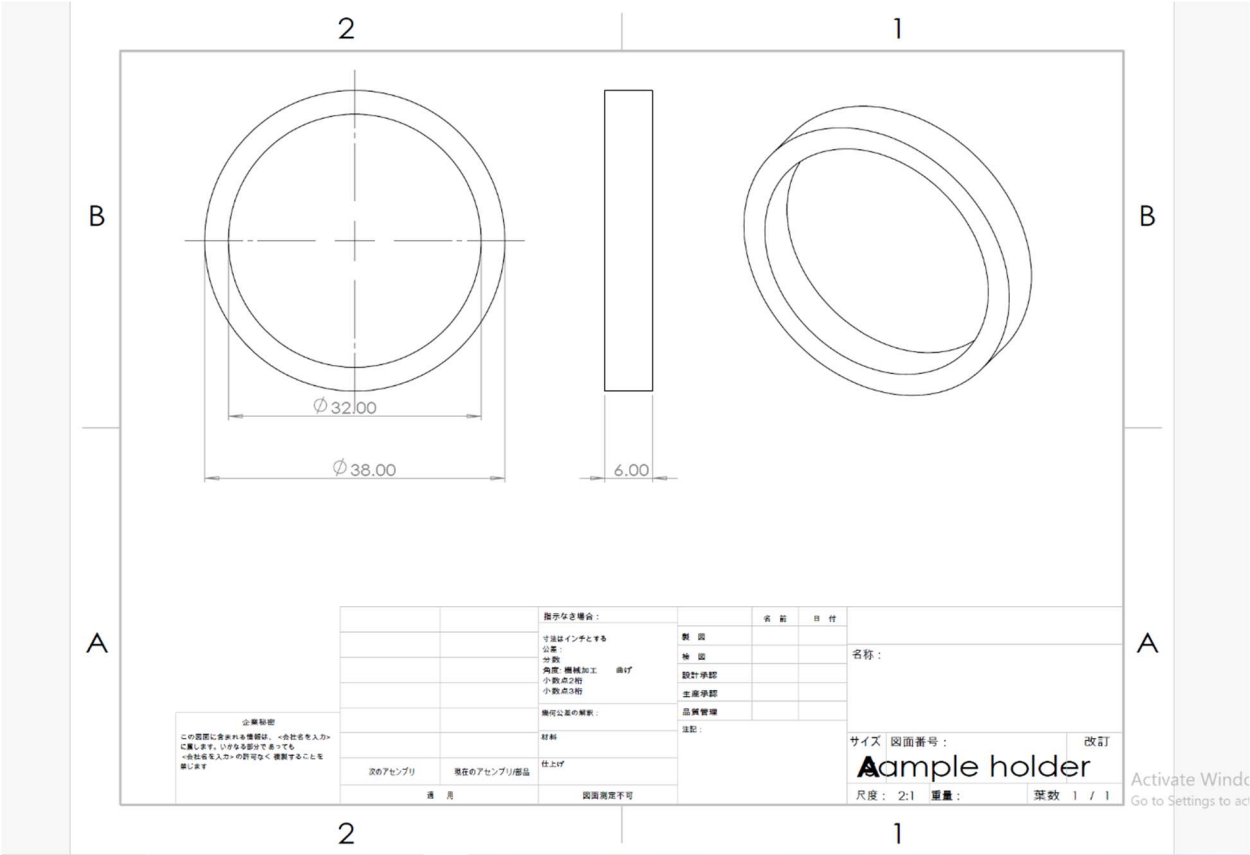
Fig. Reference Drawing
